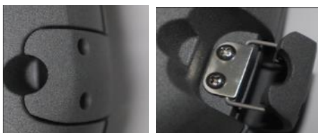
Tool free cover clips
